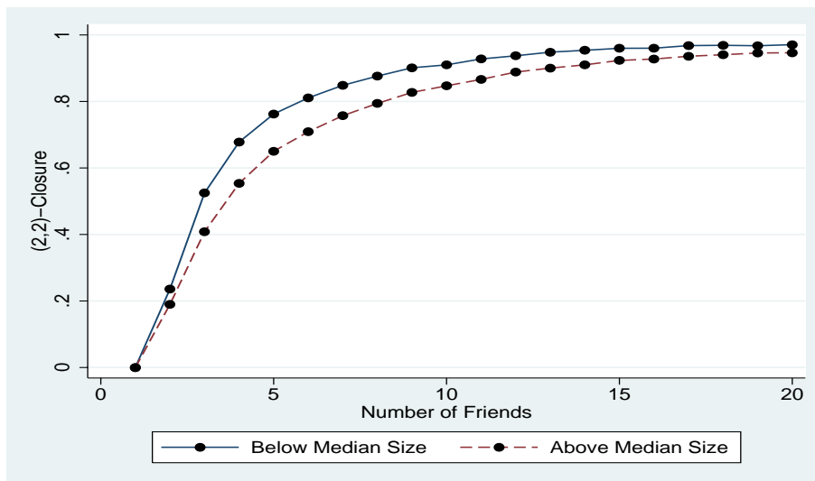
Figure 2: Mean (2, 2) -closure by number of friends for schools with grade size below median size (solid line) and schools with grade size above median size (dashed). See the text for definition of (2, 2) -closure.
